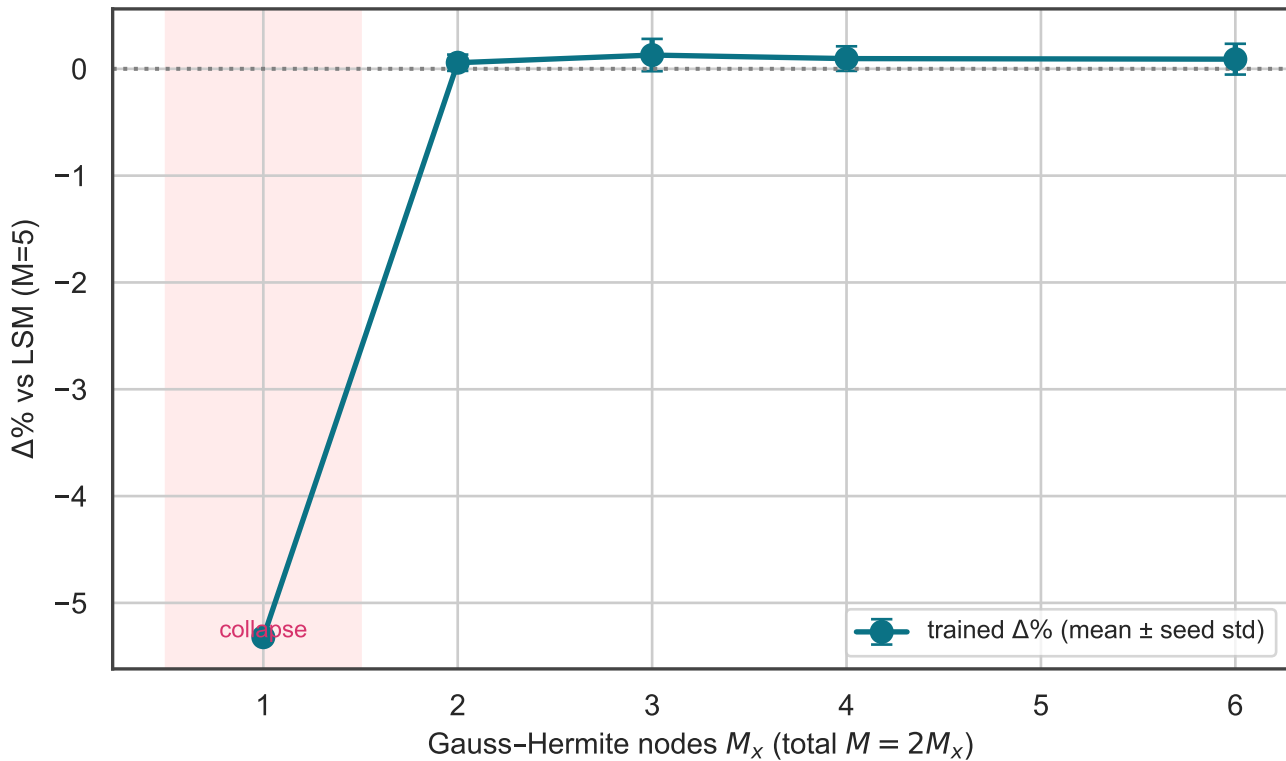
R5 · M_x isolation in the trained RL-kernel policy (focal, 4 096 ep)
